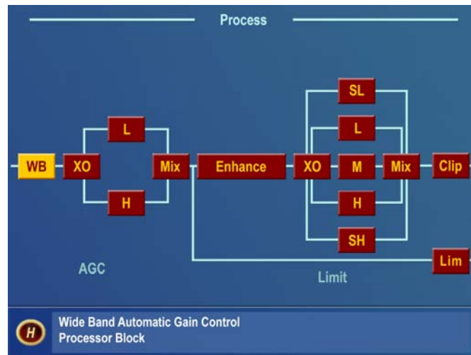
Process Submenu showing Processing Signal Chain
